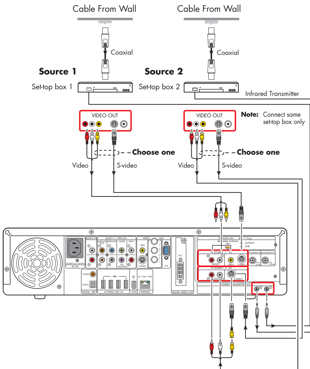
TV signal source – two digital cable boxes
